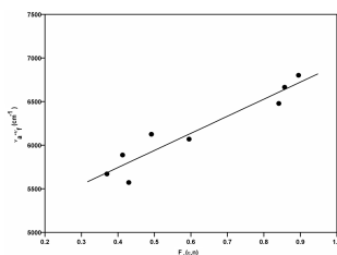
Linear fit of (\nu_\sigma - \nu_\gamma) vs. F_1(\epsilon, n) of 7-hydroxy-4-trifluoromethyl coumarin, 7H4TFMC
