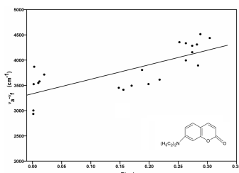
Plot of stokes shift \nu_a - \nu_f ( \text{cm}^{-1} ) versus F(\epsilon, n) of 7-diethylamino coumarin
